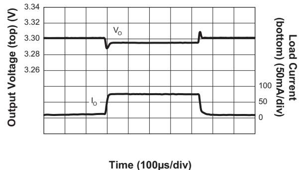
Load Transient Response (10mA to 75mA; V_{BAT} = 3.6V ; V_{OUT} = 3.3V ; C_{OUT} = 4.7\mu F )
