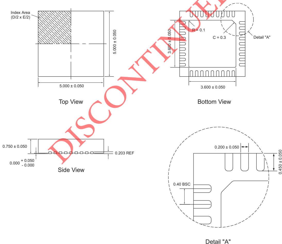
TQFN55-36 3
